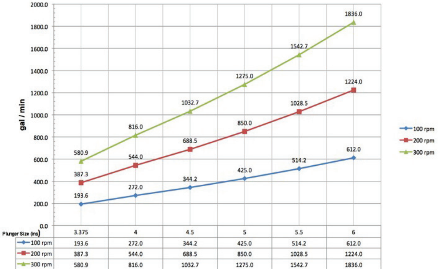
Flowrate / Plunger Size / RPM
